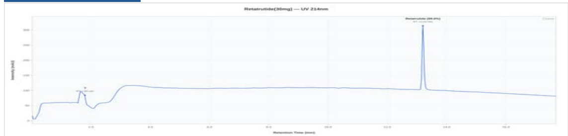
GLP3-RETA 30mg - 129-01-DK: UV Chromatogram
